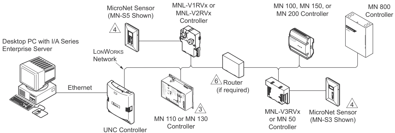
Figure-1 I/A Series MicroNet MN VAV Series Controller Connectivity.
