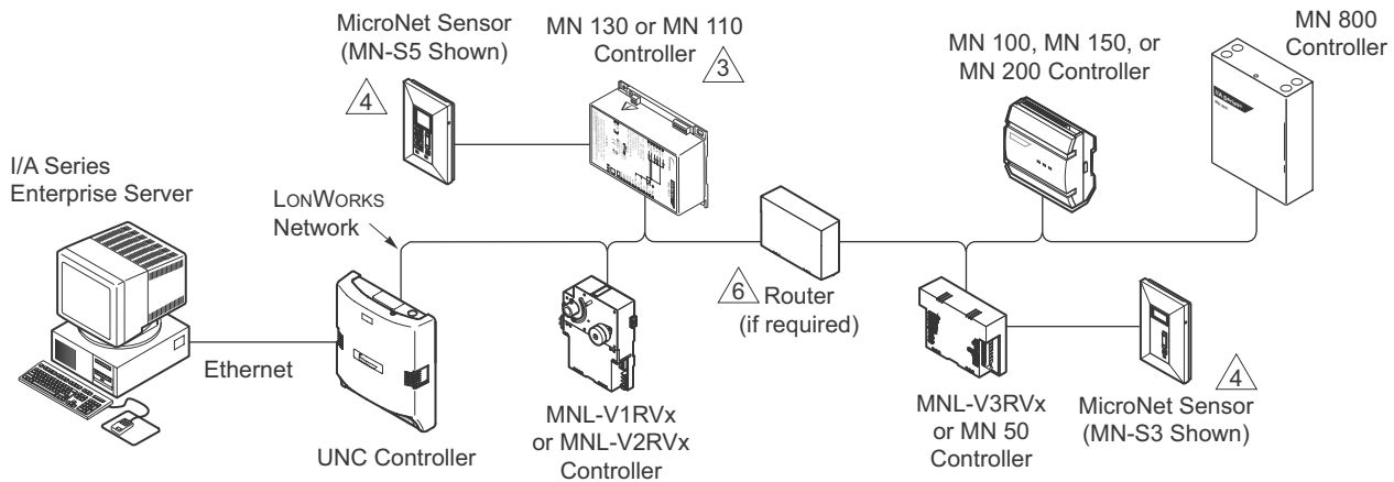
Figure-1 I/A Series MicroNet MN 110 and 130 Controller Connectivity.
